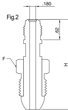
FACESEAL MALE
